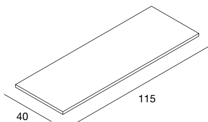
8ME/L mensola in nobilitato lucido shelf in glossy faced panel L115 x P40 cm – sp 18 mm
