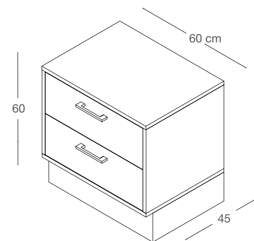
DGCS60 / L - N cassettiera in nobilitato chest of drawers in faced panel L60 x P45 x H60 cm
