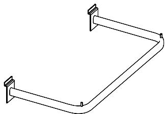
DGBAP / S - W - B barra appenderia straight hanging rail tubo ovale/oval tube 3 x 1,5 cm lungh./length: 60-90 cm
