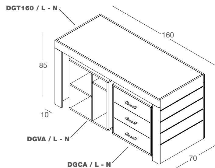
composizione banco cassa L160 con cassettiera e modulo vani in nobilitato cash counter unit L160 with chest of drawers and compartment in faced panel L160 x P70 x H85 cm
