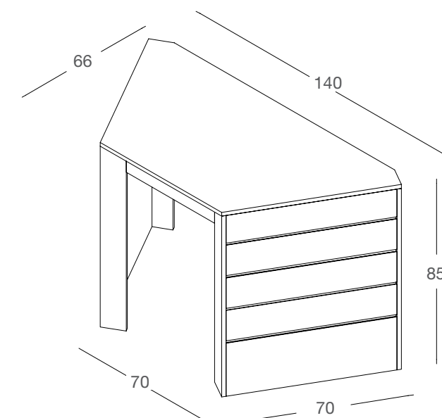
DGT140 / L - N tavolo trapezio con fianchi dogati in nobilitato trapezoid-shaped table with slat-panel sides in faced panel L140 x P66 x H85 cm
