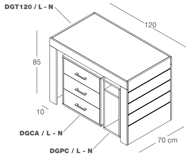
composizione banco cassa L120 con cassettiera e porta pc in nobilitato cash counter unit L120 with chest of drawers and pc holder in faced panel L120 x P70 x H85 cm
