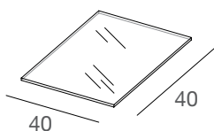
DGMEM / V mensola in vetro temperato shelf in tempered glass L40 x P40 x SP0,8 cm
