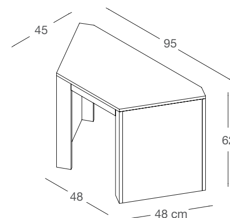
DGT95 / L - N tavolino trapezio in nobilitato trapezoid-shaped small table in faced panel L95 x P45 x H62 cm
